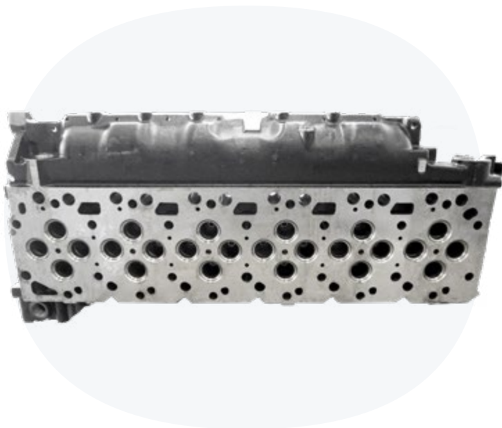
WITHOUT VALVES
